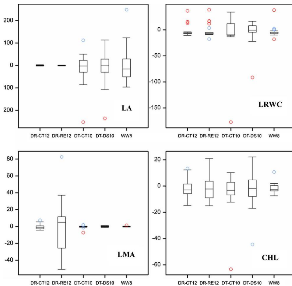
Fig. 2. Spread in SCA effects of crosses for selected traits at different watering conditions LA, leaf area; LRWC, leaf relative water content; LMA, leaf mass area; CHL, chlorophyll content.
